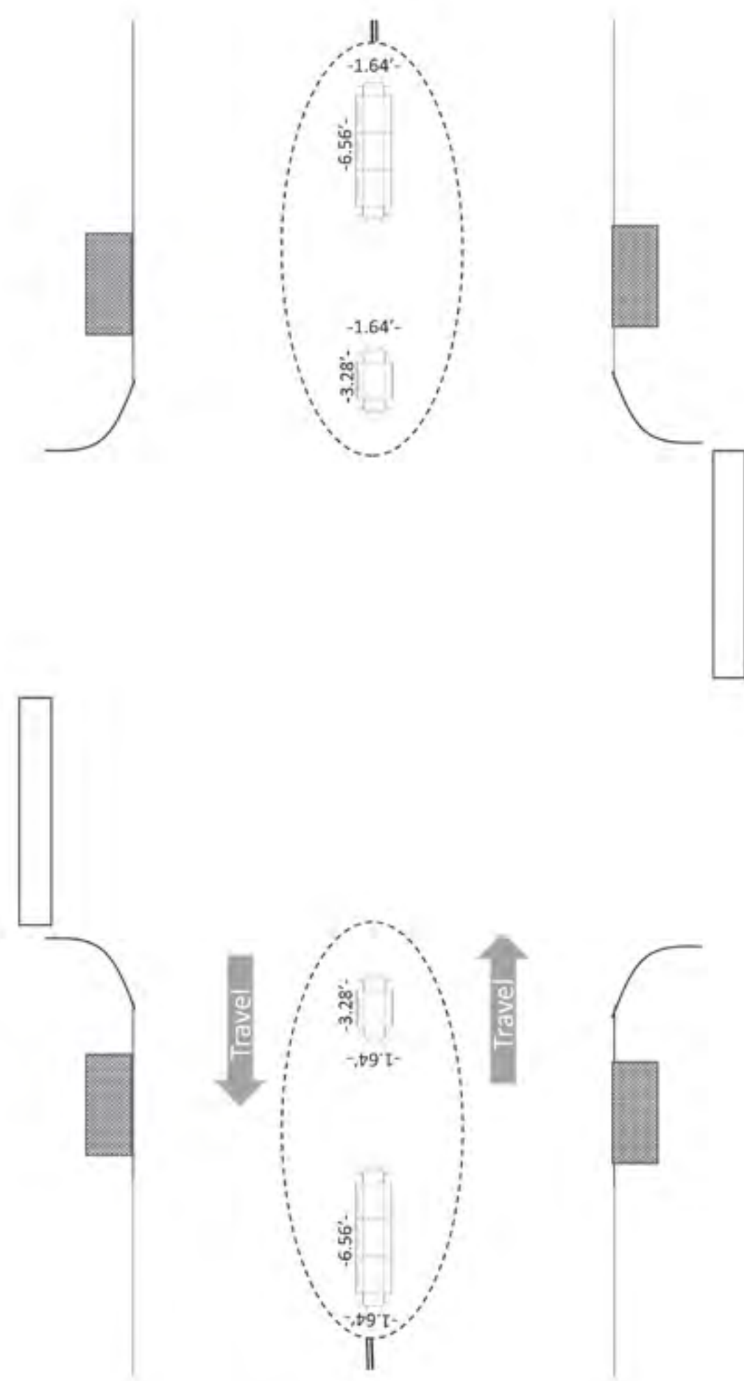
Full Mini-Pedestrian Refuge Median @ Intersection
