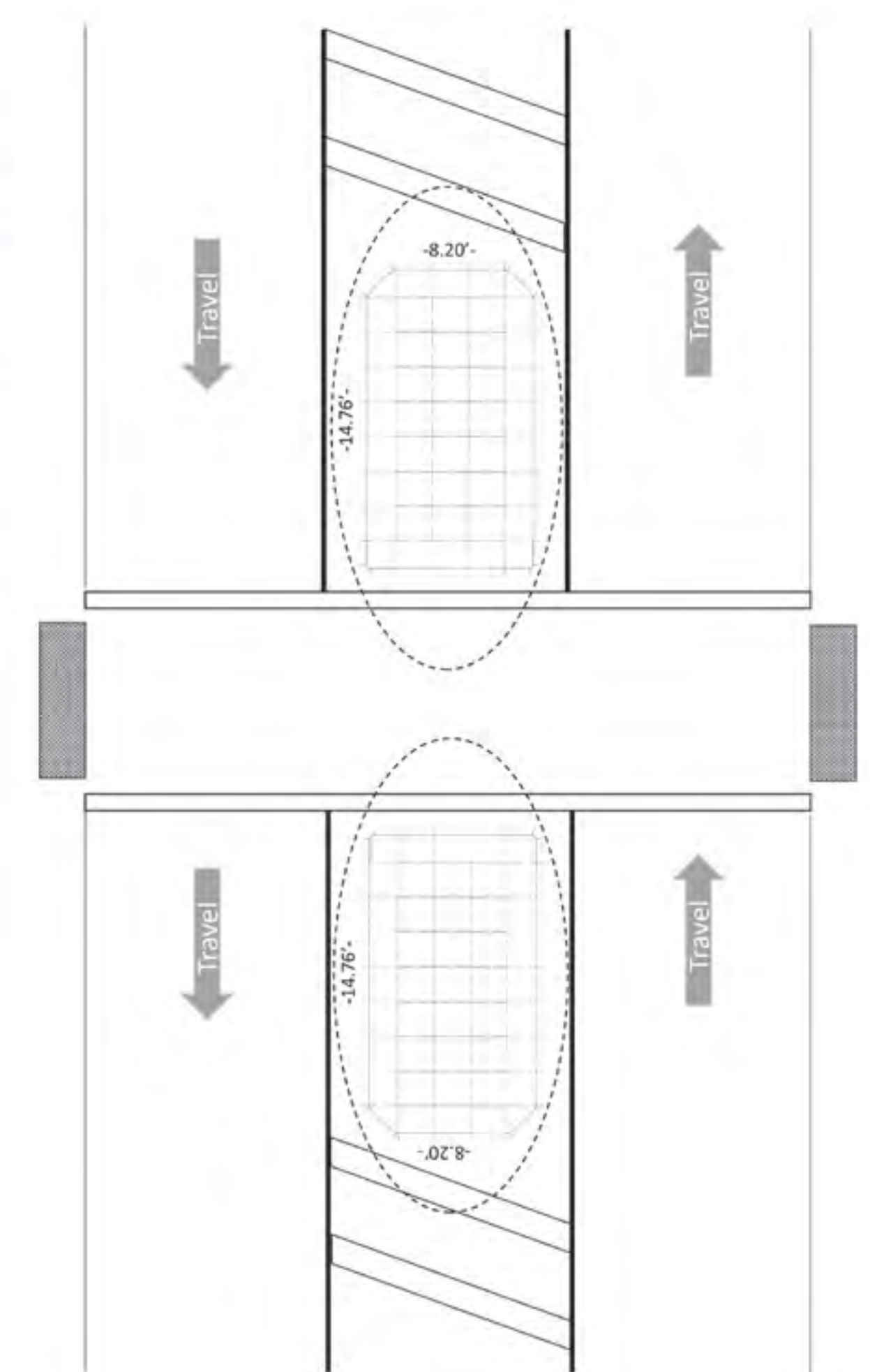
Full Pedestrian Refuge Median @ Mid-Block
